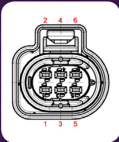
Bosch LSU4.9 Sensor Diagram
